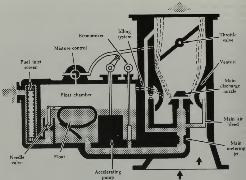
FIGURE 3-7. A float-type carburetor.
